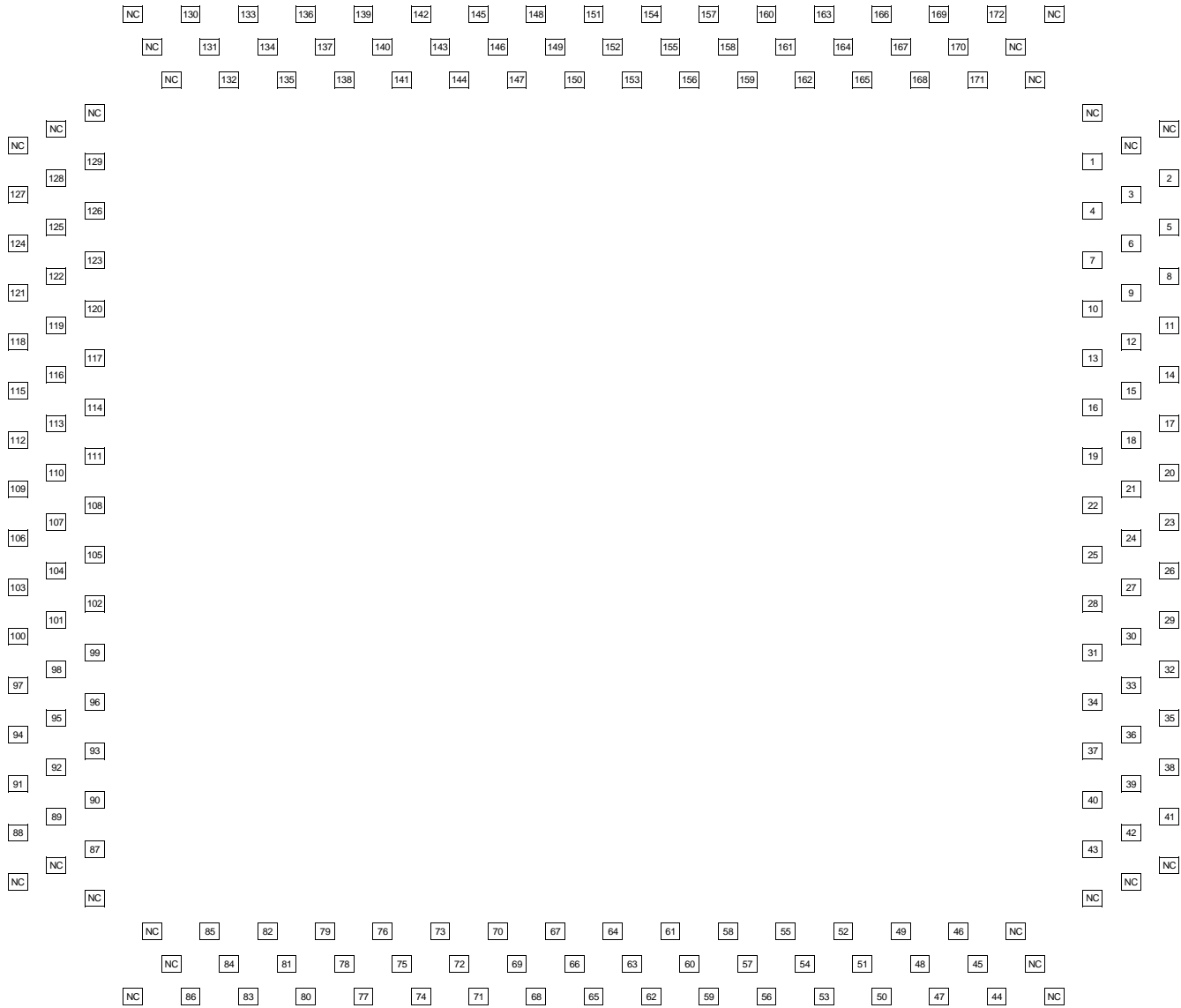
SY-CQ196 Pin Assignment with 172-pin CQFP Top View
